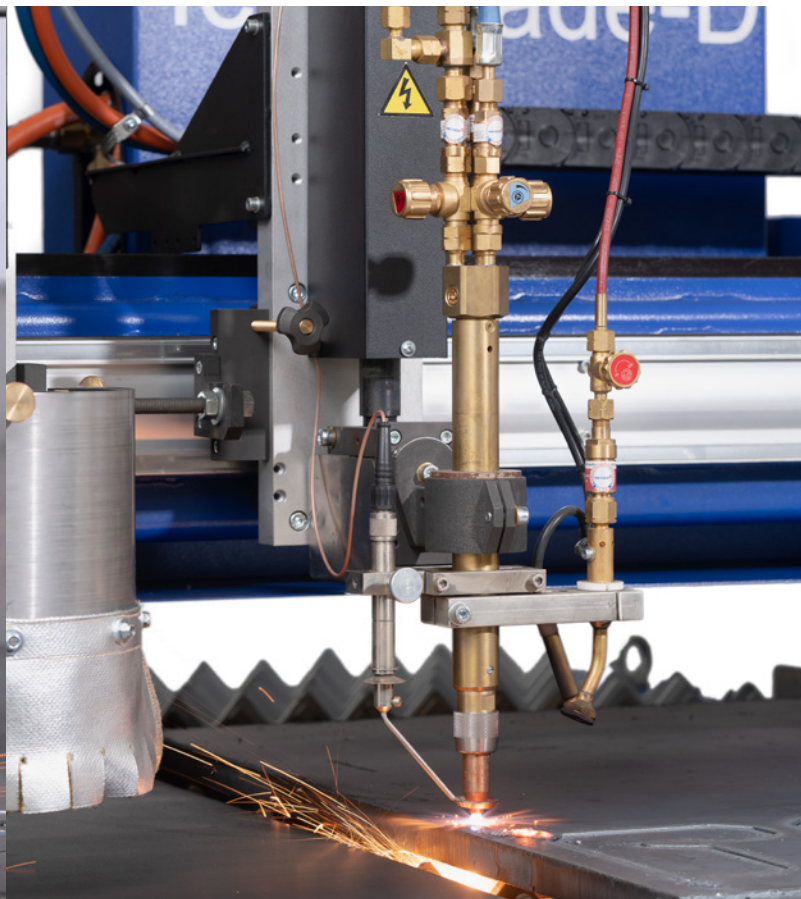
Excellent and cost-effective oxyfuel cuts
